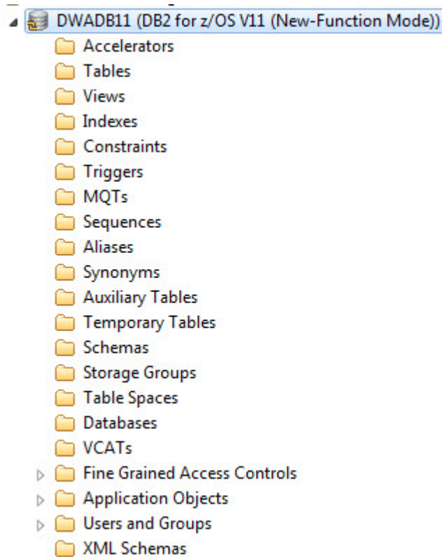
Figure 8. Database server connection in the Administration Explorer
