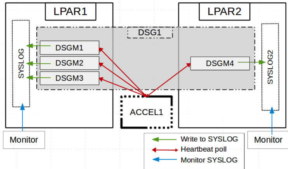
Figure 14. Members in two different LPARs
