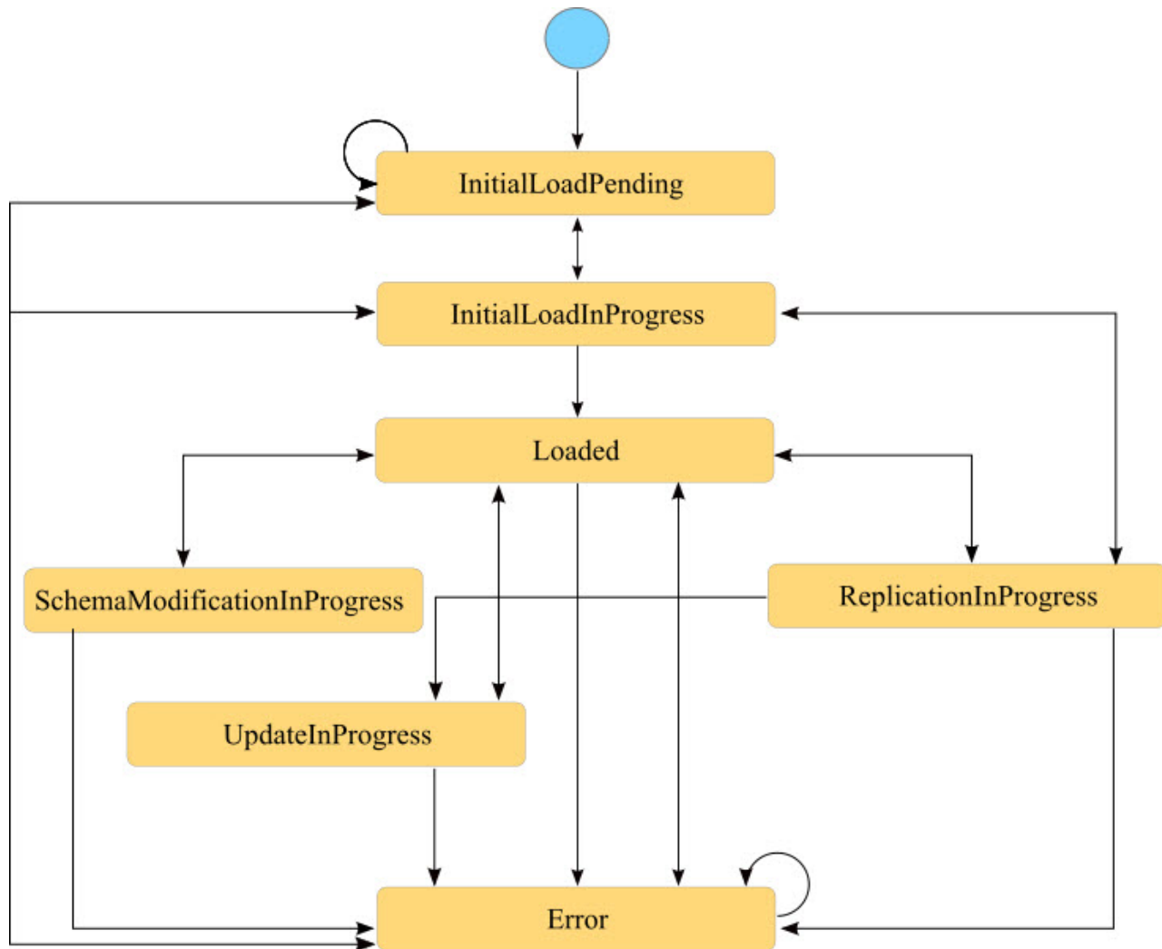
Figure 3. Possible table state transitions
