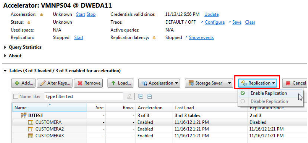
Figure 11. Timestamp columns and Replication button in the accelerator view
