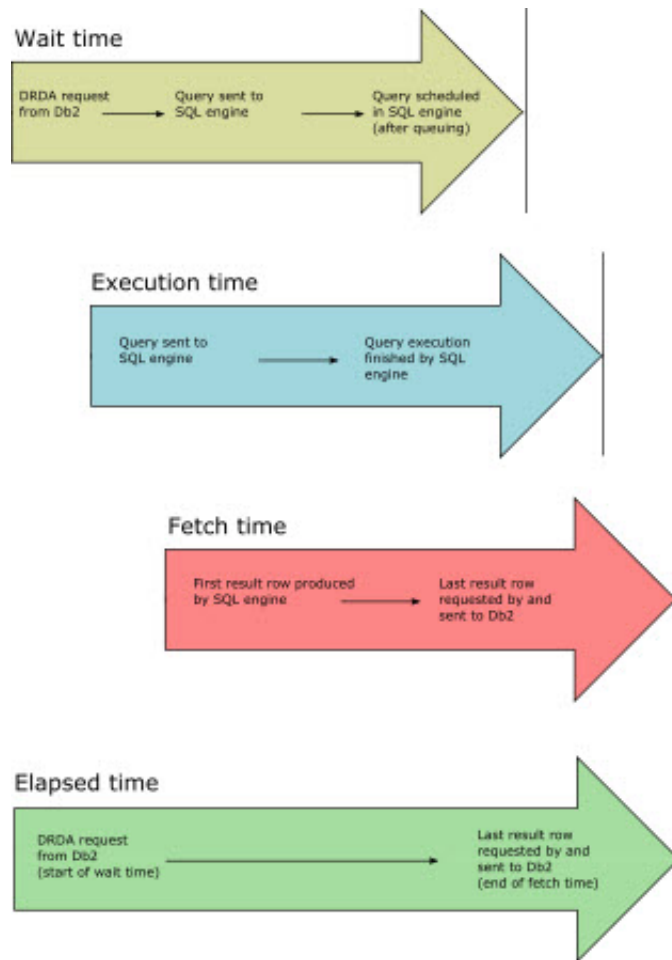
Figure 9. Wait time, execution time, fetch time, and elapsed time in comparison
